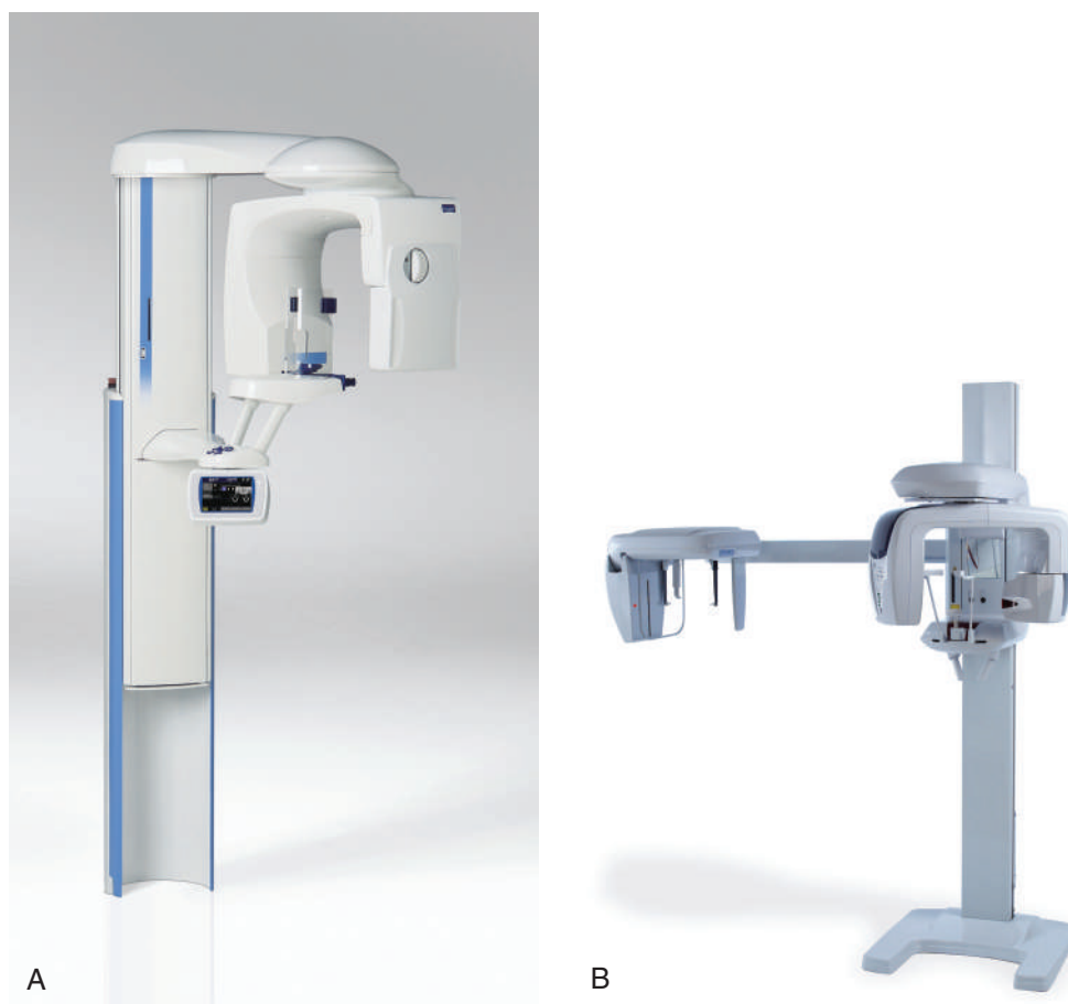
Fig. 2.6 A , Planmeca ProMax 3D. B , J. Morita Veraviewepocs 3D. (A, Courtesy Planmeca Oy, Helsinki, Finland. B, Courtesy, JMorita USA, Irvine, CA).
